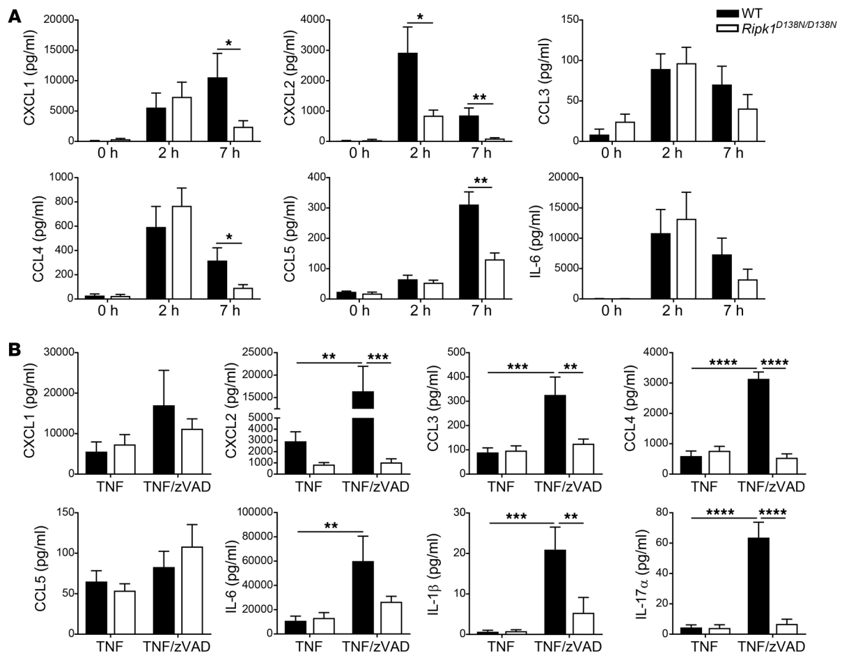
Figure 1. Ripk1 D138N/D138N mice exhibit impaired cytokine and chemokine production in response to TNF and TNF/zVAD administration in vivo. (A) Plasma cytokine and chemokine levels in WT and Ripk1 D138N/D138N mice 2 and 7 hours after i.v. TNF administration ( n = 8-9 ) or (B) 2 hours after i.v. TNF or TNF/zVAD administration ( n = 6-9 ). TNF-induced levels are repeated from A. Data are shown as mean \pm SEM. * P < 0.05 ; ** P < 0.01 ; *** P < 0.001 ; **** P < 0.0001 , 2-tailed Student's t test (A) or 2-way ANOVA with post hoc Tukey's test (B).
