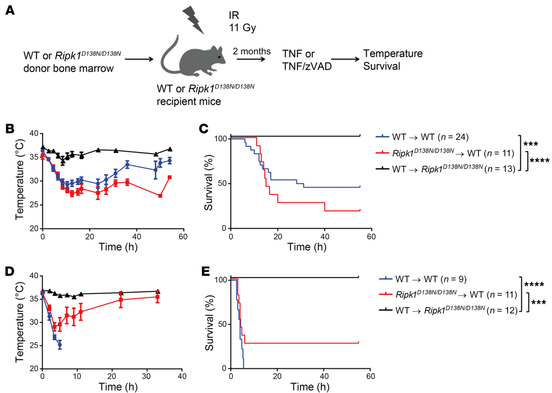
Figure 3. Nonhematopoietic RIPK1 kinase-inactive cells protect against TNF- and TNF/zVAD-induced shock. (A) Experimental design. IR, irradiation. Body temperature (B and D) and Kaplan-Meier survival curves (C and E) after TNF- (B and C) or TNF/zVAD-induced shock (D and E) are depicted for lethally irradiated WT and Ripk1 D138N/D138N mice reconstituted with WT or Ripk1 D138N/D138N bone marrow cells. Data are shown as mean ± SEM. *** P < 0.001; **** P < 0.0001, Mantel-Cox test.
