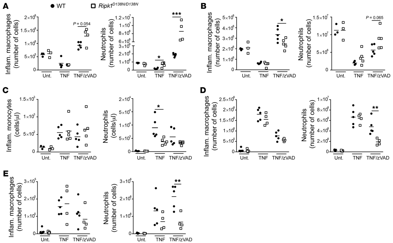
Figure 2. Impaired recruitment of Ripk1 D138N/D138N inflammatory cells in response to TNF or TNF/zVAD administration. (A and B) Splenocytes and bone marrow cells were stained with antibodies, analyzed by flow cytometry, and the number of inflammatory (Inflam.) monocytes/macrophages or neutrophils determined. The number of cells for WT and Ripk1 D138N/D138N mice left untreated (Unt.) or treated with TNF (7 hours) or TNF/zVAD (4 hours) ( n = 3-5 ) is shown. (C) The number of inflammatory monocytes or neutrophils in peripheral blood of WT and Ripk1 D138N/D138N mice left untreated or treated with TNF (7 hours) or TNF/zVAD (4 hours) is shown ( n = 3-5 ). (D and E) The number of inflammatory macrophages or neutrophils in lung and liver of WT and Ripk1 D138N/D138N mice left untreated or treated with TNF (7 hours) or TNF/zVAD (4 hours) ( n = 4-5 ) is shown. * P < 0.05 ; ** P < 0.01 ; *** P < 0.001 , 2-tailed Student's t test.
