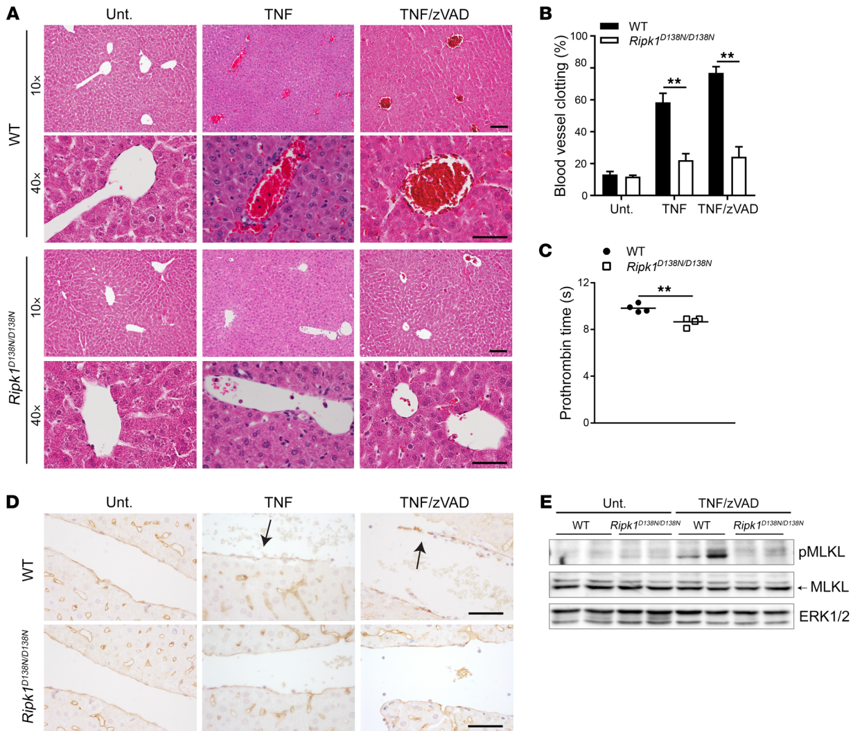
Figure 6. RIPK1 kinase-inactive mice are protected from TNF- or TNF/zVAD-induced coagulation and breaks in the liver endothelium, and from TNF/zVAD-induced liver endothelial cell necrosis. (A) Representative images of H&E-stained liver sections from WT or Ripk1 D138N/D138N mice left untreated or injected i.v. with TNF or TNF/zVAD ( n = 3-4 mice). Scale bars: 100 \mu\text{m} ( \times 10 ); 50 \mu\text{m} ( \times 40 ). (B) Quantification of clotting observed in liver blood vessels of mice shown in A. (C) Citrated plasma was isolated from WT and Ripk1 D138N/D138N mice 7 hours after TNF administration, and clot formation time was measured by the prothrombin time test ( n = 4 mice). (D) Representative images of endomucin-stained liver sections from untreated or TNF- or TNF/zVAD-treated WT and Ripk1 D138N/D138N mice ( n = 3-4 mice). Scale bars: 50 \mu\text{m} ( \times 40 ). (E) WT and Ripk1 D138N/D138N liver endothelial cells were isolated from untreated or TNF/zVAD-treated mice. A representative Western blot showing protein lysates probed with antibodies to phospho-MLKL, MLKL, and ERK1/2 is depicted. Lysates were generated and analyzed from 14 WT and 8 Ripk1 D138N/D138N TNF/zVAD-treated mice. Data are shown as mean \pm SEM. ** P < 0.01 , 2-tailed Student's t test.
