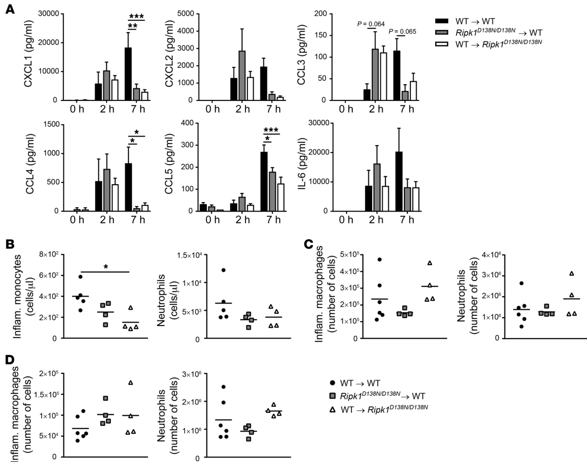
Figure 4. Proinflammatory cytokines and inflammatory cell recruitment do not correlate with survival in a TNF-induced model of shock. (A) Plasma cytokine and chemokine levels in reconstituted mice 2 and 7 hours after i.v. TNF administration ( n = 4-7 ). Graphs depicting the number of inflammatory monocytes/macrophages and neutrophils in the blood (B), lungs (C), or liver (D) of lethally irradiated WT and Ripk1 D138N/D138N mice reconstituted with WT or Ripk1 D138N/D138N bone marrow cells as measured by flow cytometry 8 hours after systemic TNF administration ( n = 4-5 ). Data are shown as mean \pm SEM. * P < 0.05 ; ** P < 0.01 ; *** P < 0.001 , 2-way (A) or 1-way ANOVA with post hoc Tukey's test (B-D).
