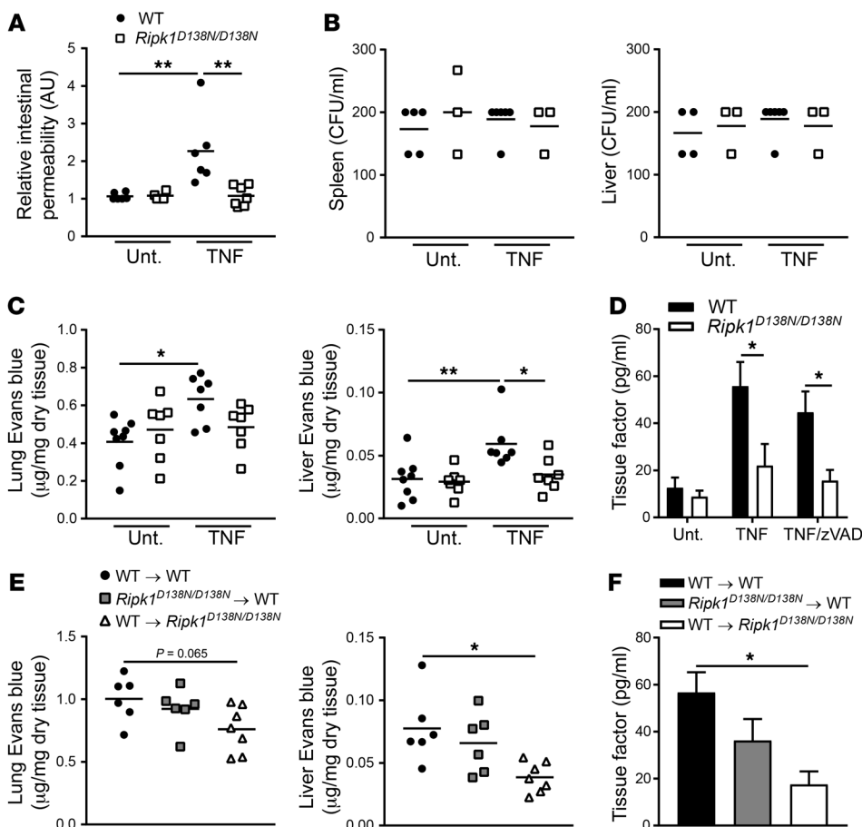
Figure 5. Nonhematopoietic RIPK1 kinase-inactive cells protect against TNF-induced intestinal and vascular hyperpermeability and coagulation. (A) FITC-labeled dextran beads were administered to WT and Ripk1 D138N/D138N mice by oral gavage 2 hours after TNF injection. Blood was isolated by cardiac puncture and the levels of FITC-dextran in plasma measured by fluorometry ( n = 4-7 ). (B) Bacterial growth in spleen and liver lysates isolated from untreated WT and Ripk1 D138N/D138N mice or 10 hours after injection with 15 \mu g TNF ( n = 3-6 ). (C) WT and Ripk1 D138N/D138N mice were injected with TNF and Evans blue dye, organs were collected, and the amount of dye extracted from the lung and liver was measured by spectrophotometry ( n = 7-8 ). (D) Tissue factor levels were determined by ELISA in the plasma of TNF- or TNF/zVAD-treated WT and Ripk1 D138N/D138N mice ( n = 3-7 ). (E) WT and Ripk1 D138N/D138N reconstituted mice were injected with TNF and Evans blue dye, and the amount of dye extracted from the lung and liver was measured by spectrophotometry ( n = 6-7 ). (F) Tissue factor levels in the plasma of reconstituted WT and Ripk1 D138N/D138N mice treated with TNF ( n = 3-5 ). Data are shown as mean \pm SEM. * P < 0.05 ; ** P < 0.01 , 2-way ANOVA with post hoc Tukey's test (A and C), 2-tailed Student's t test (D), or 1-way ANOVA with post hoc Tukey's test (E and F).
