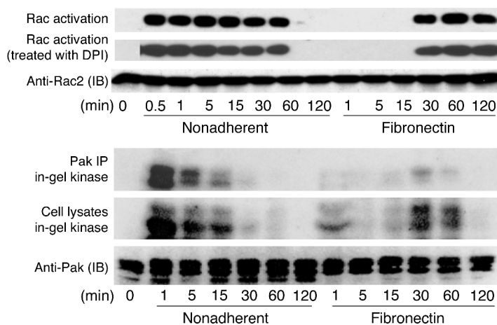
Figure 2 Adhesion of neutrophils to fibronectin leads to delayed Rac2 and Pak activation in response to fMLF stimulation. Neutrophils plated on fibronectin (50 \mu\text{g}/\text{ml} ) or in nonadherent conditions were treated with 1 \times 10^{-7} M fMLF. After the times indicated, Rac2 activity in the absence or presence of 10 \mu\text{M} DPI was determined, as in Methods. Total Rac2 levels (anti-Rac2 IB) did not change with time under each condition. Pak1 and Pak2 activities were analyzed by in-gel kinase assays of immunoprecipitated (IP) Pak or directly in cell lysates. IBs in the bottom panel show that Pak (1 and 2) levels did not change with time under each condition. The results shown are representative of four similar experiments obtained with cells derived from different donors.
