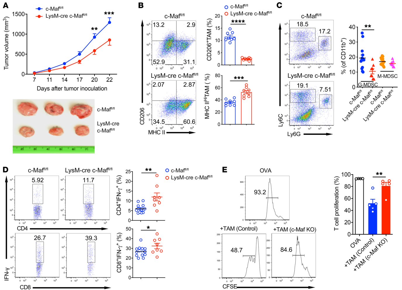
Figure 7. Deletion of c-Maf in myeloid cells suppresses tumor growth with enhanced antitumor T cell responses. (A) c-Maf fl/fl control ( n = 14 ) and LysM-cre c-Maf fl/fl mice ( n = 8 ) were inoculated with LLC cells s.c., and tumor growth was monitored (upper). Representative tumor pictures are shown (lower). **P < 0.01 , ***P < 0.001 by 2-way repeated-measures ANOVA with Sidak's multiple-comparisons test. (B) TAMs were stained for CD206 and MHC II expression. Cells were gated on CD11b + Gr-1 - F4/80 + viable cells. Representative dot plots and summarized percentages of cells are shown. (C) Representative MDSC populations by flow cytometry and summarized frequencies are shown. Cells were gated on CD11b + viable cells. (D) Single-cell suspensions from tumors were stimulated with PMA plus ionomycin and intracellular IFN- \gamma staining was performed. Representative dot plots and summarized data are shown. Cells were gated on CD4 + or CD8 + T cells. (E) TAMs from control and c-Maf-KO mice were cocultured with CFSE-labeled splenocytes from OVA-Tg OT-I mice in the presence of OVA. T cell proliferation was analyzed. Cells were gated on CD8 + cells. Representative histograms and percentage of proliferated cells are shown. Data are shown as mean \pm SEM. *P < 0.05 ; **P < 0.01 ; ***P < 0.001 ; ****P < 0.0001 by 2-tailed, unpaired t test (B-D); **P < 0.01 by 1-way ANOVA with post hoc t test and Bonferroni's correction (E).
