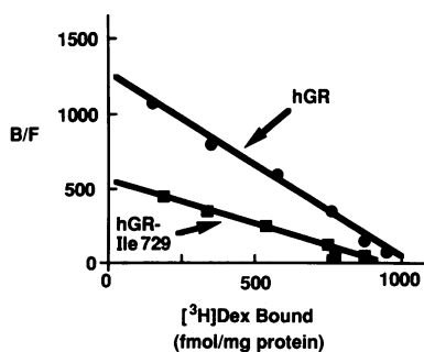
Figure 6. Scatchard analysis of [ ^3 H]Dex binding to the wild-type hGR and hGR-Ile 729. COS-1 cells were transfected with the wild-type hGR or hGR-Ile 729 expression vector using the DEAE-dextran method, and the cytosol was assayed for [ ^3 H]Dex binding. Cytosol from control COS-1
