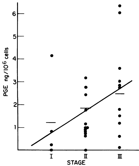
FIGURE 3 PGE levels measured by radioimmunoassay are plotted as a function of stage of disease. ●, PGE levels from the mononuclear cell cultures of 27 individual patients whose cells were cultured in autologous serum. The straight line curve fitted by linear regression analysis has a correlation coefficient of r = 0.42 , P < 0.05 . The horizontal bar represents the mean at each stage.
